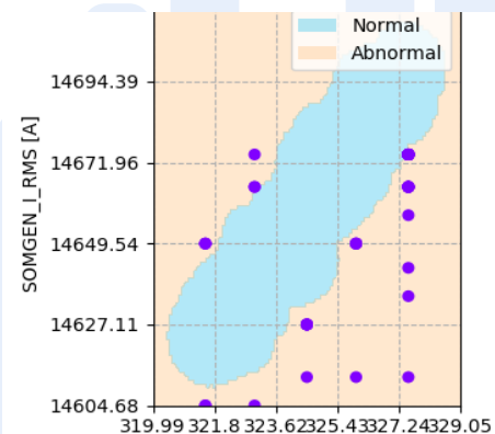
Anomaly Detection Map: Purple Marking Signal System Anomalies
